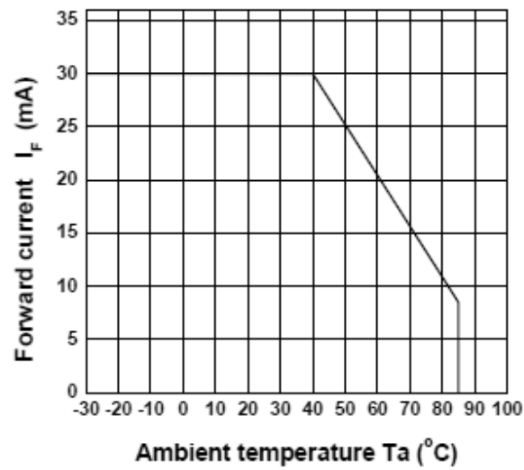
Diode IF-Ta CHARACTERISTICS DIAGRAM
