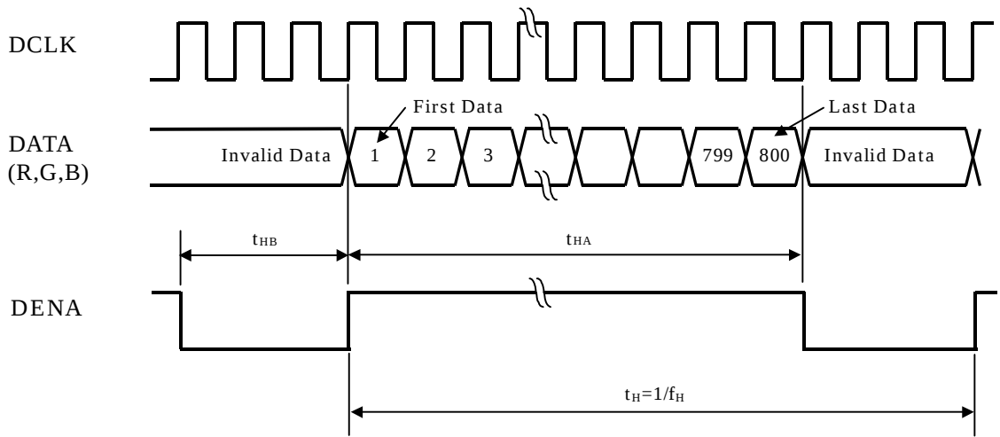
a. Horizontal Timing Chart
