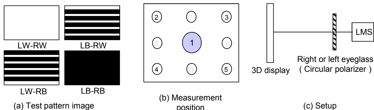
FIG. 6 Measurement configuration
