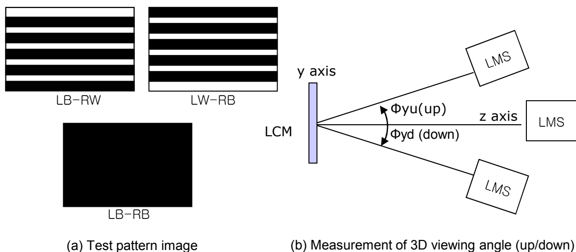
FIG. 9 Measurement of 3D crosstalk and 3D viewing angle
