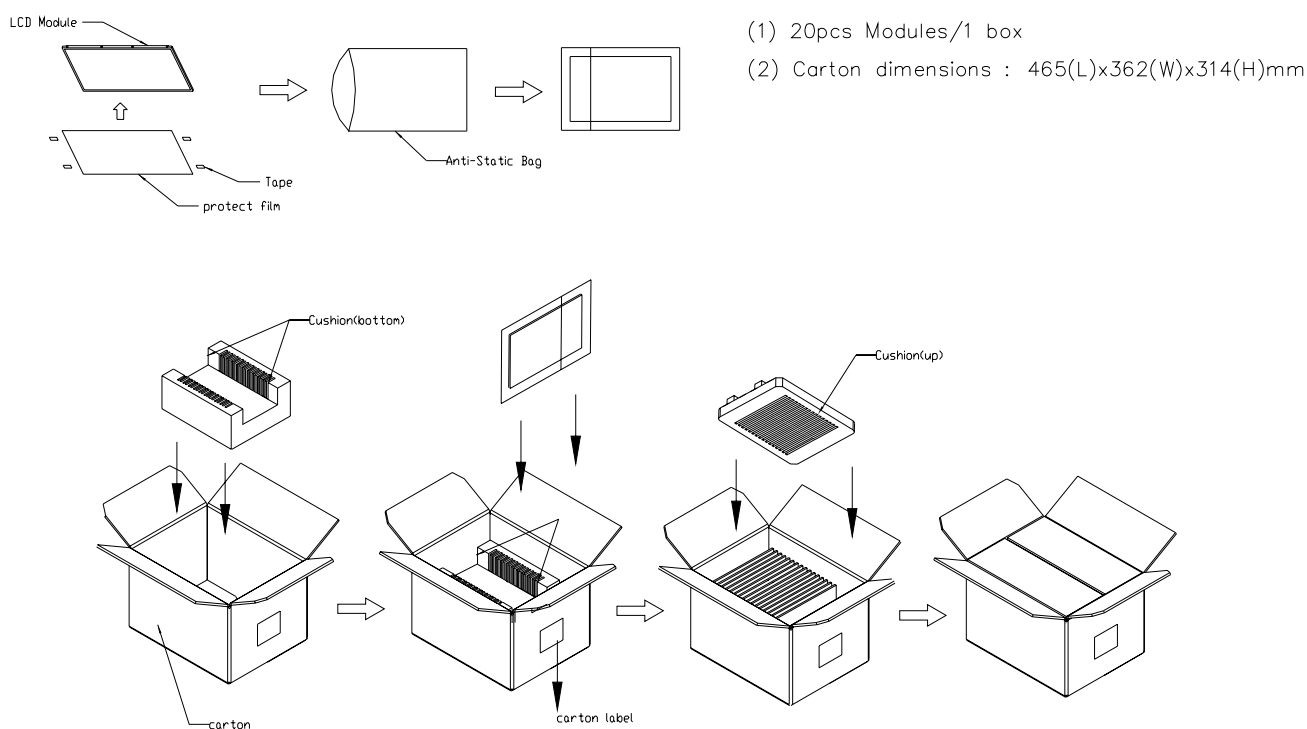
Figure. 6-1 Packing method
