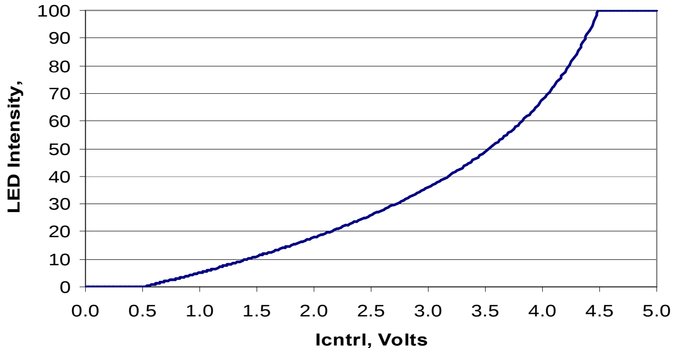
LED Intensity vs Icntrl
