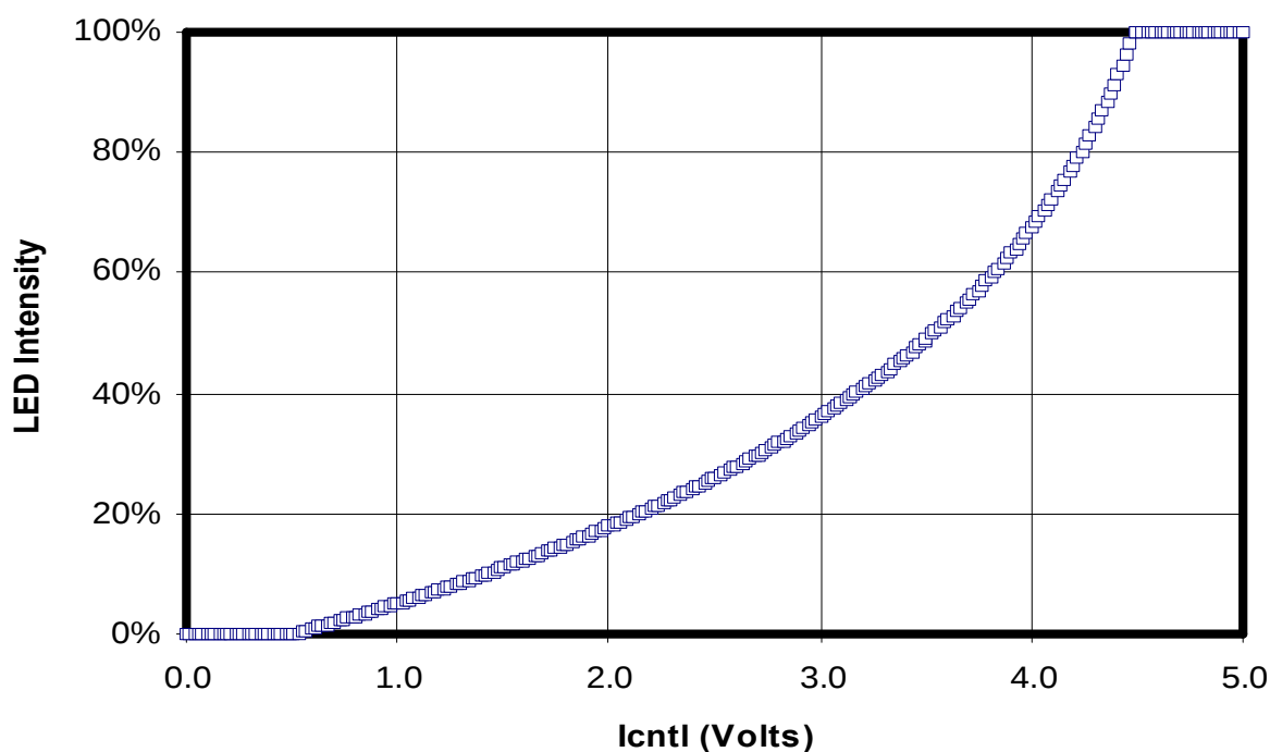
LED Intensity vs. Ictrl Voltage
