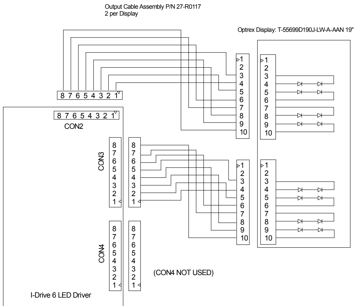
Connection Diagram
