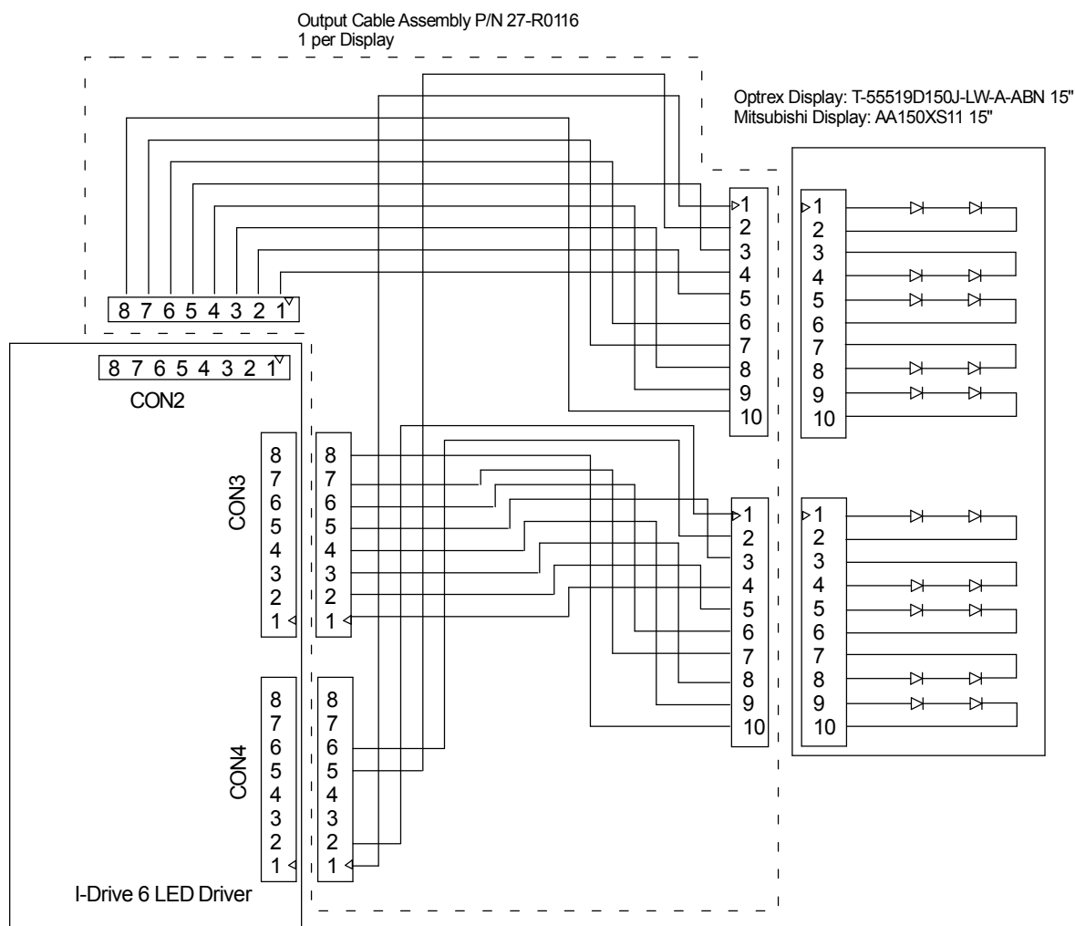
Connection Diagram
