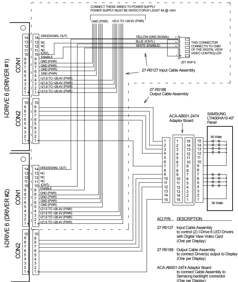
Connection Diagram (Display requires (2) I-Drive 6 LED Drivers) Display backlight power requirement = 2 x 56W = 112W
