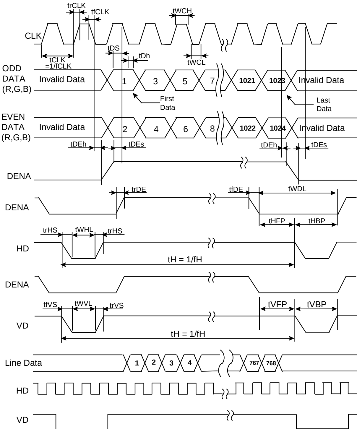
(b)Timing Chart
