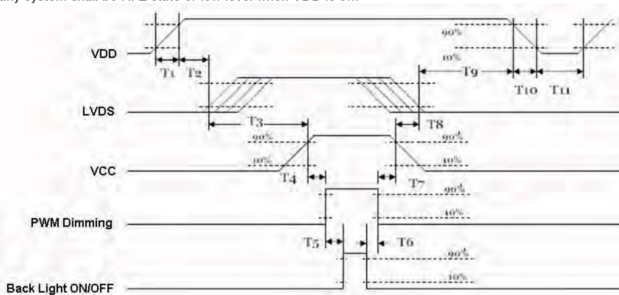
Power ON/OFF sequence timing
