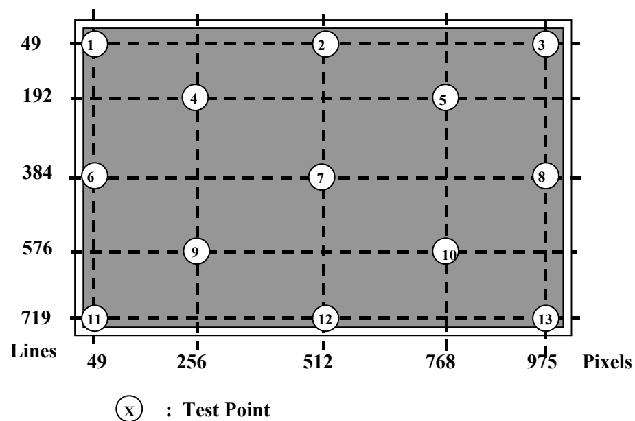
Figure 2. Average Luminance Measurement Locations & Uniformity Measurement Locations
