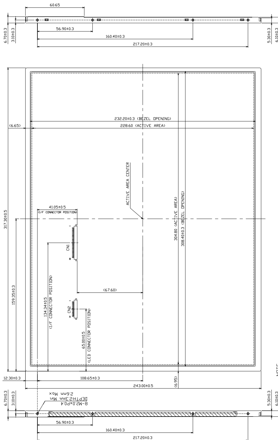
Figure 5. TFT-LCD Module Outline Dimension (Front View)
