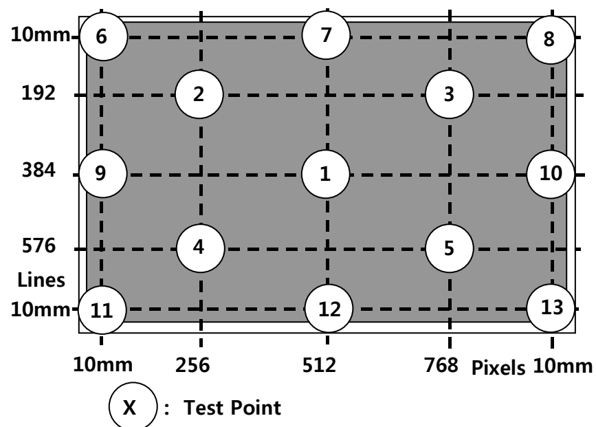
Figure 2. Average Luminance Measurement Locations & Uniformity Measurement Locations
