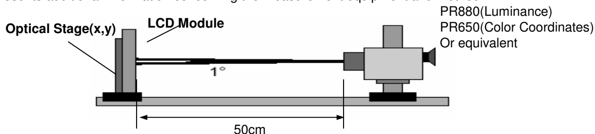
FIG. 1 Optical Characteristic Measurement Equipment and Method
