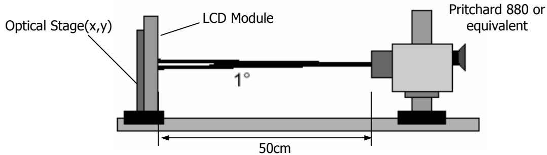
[ Figure 8 ] Optical characteristic measurement equipment and method
