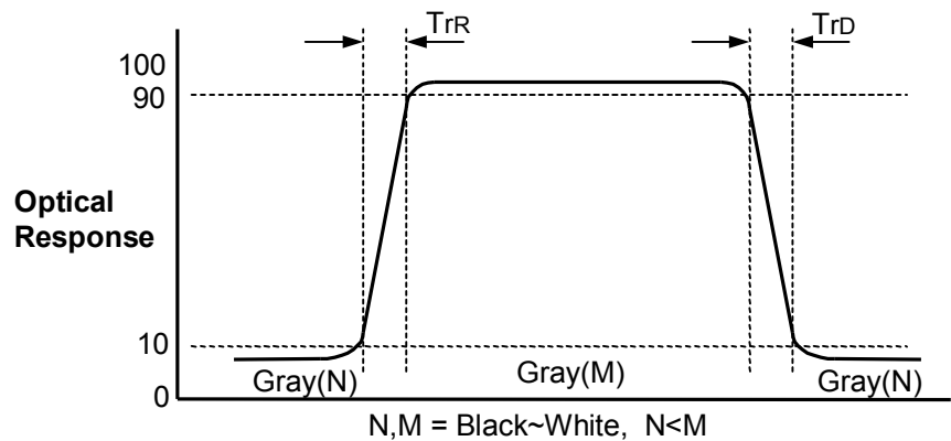
FIG. 3 Response Time
