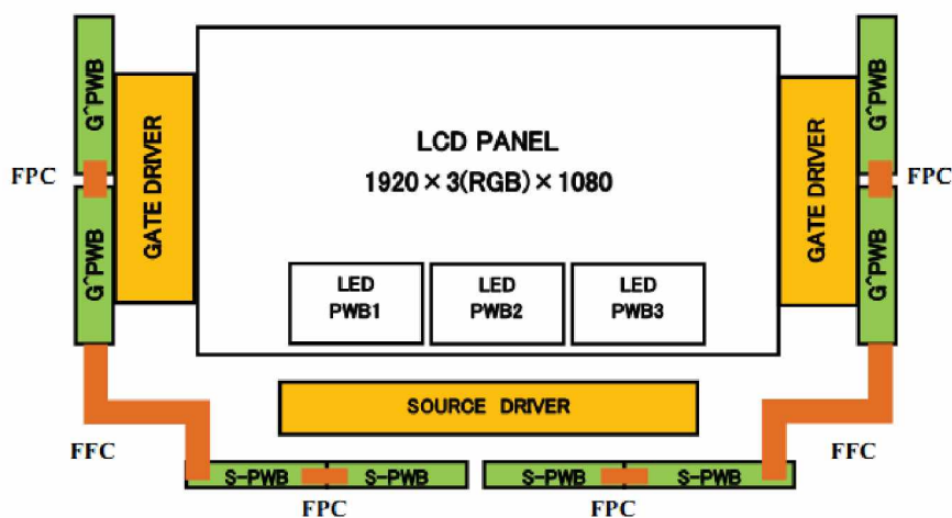
Layout of LED-PWB, S-PWB & G-PWB (Front View)
