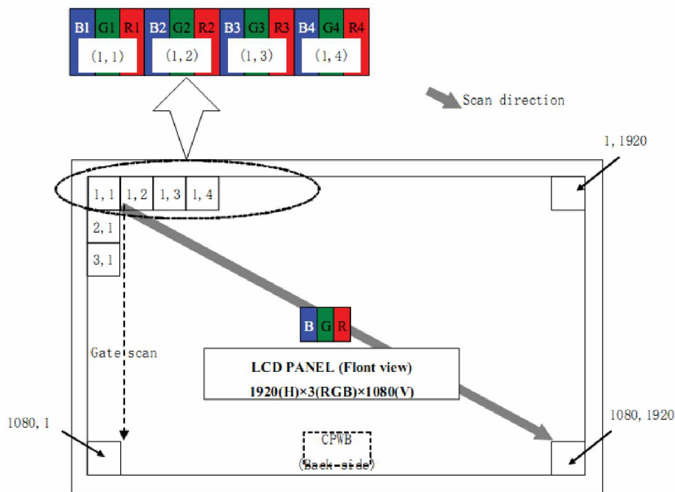
LCD subpixel alignment in Landscape installaion
