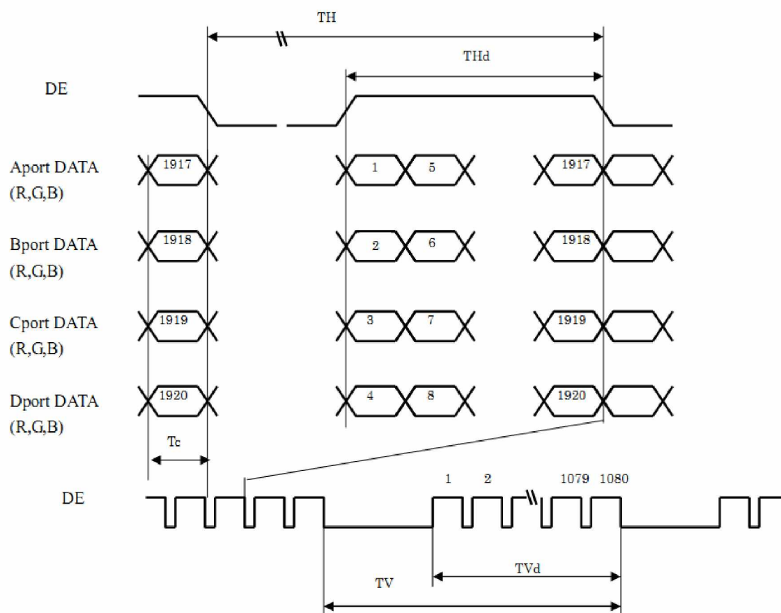
Timing characteristics of input signals
