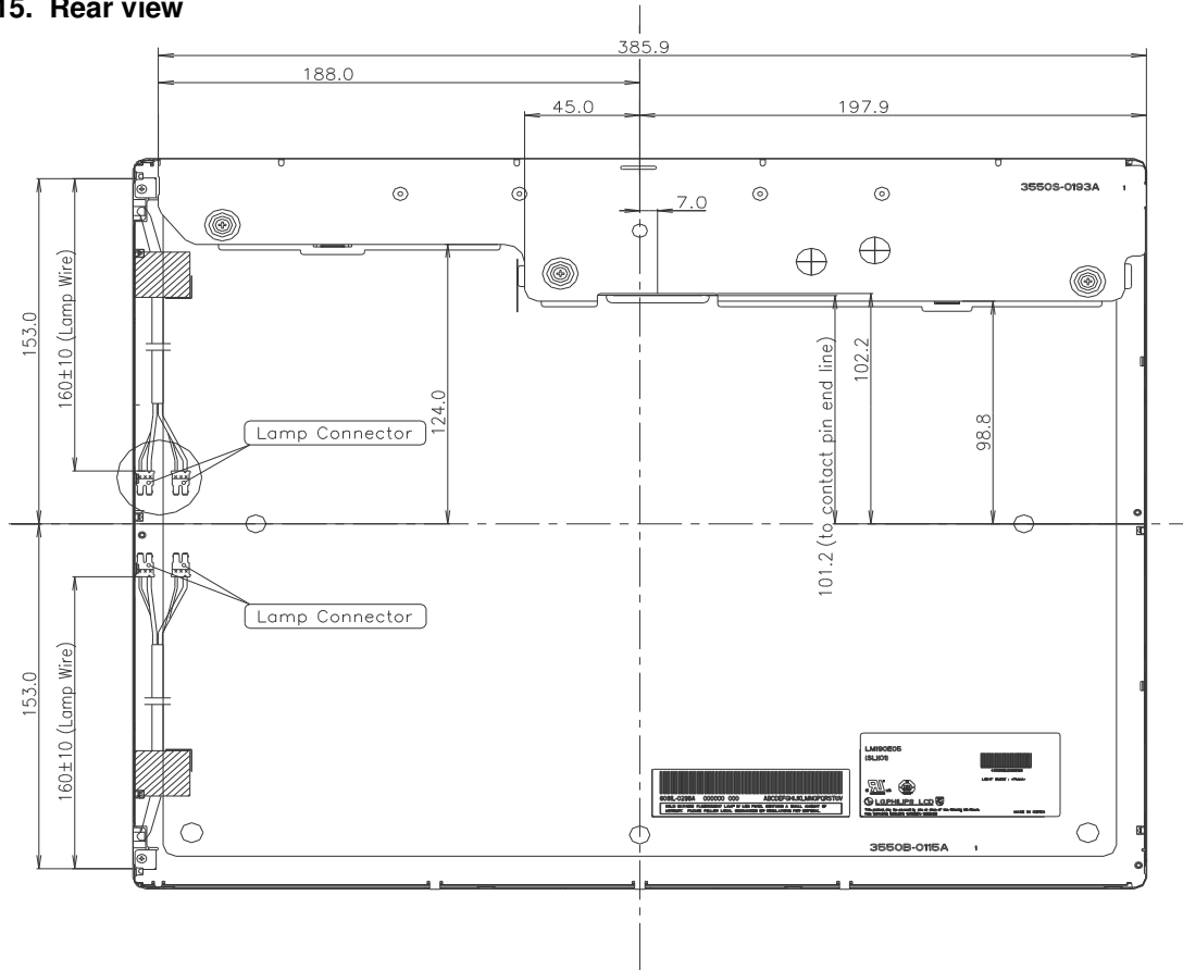
Figure 15. Rear view
