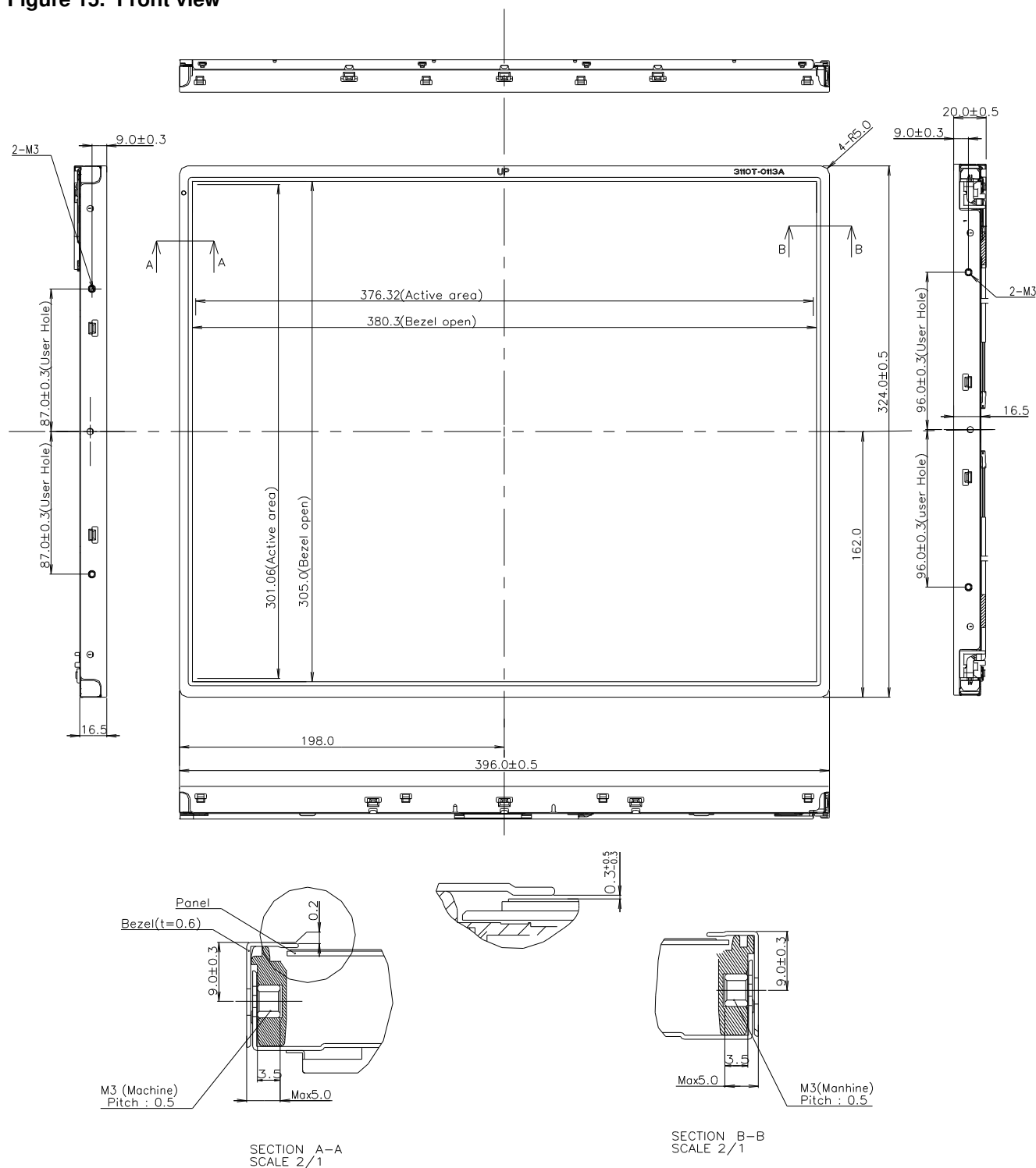
Figure 15. Front view
