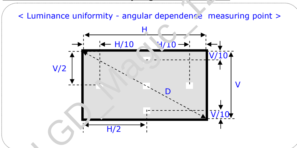
FIG. 11 Luminance Uniformity angular dependence
