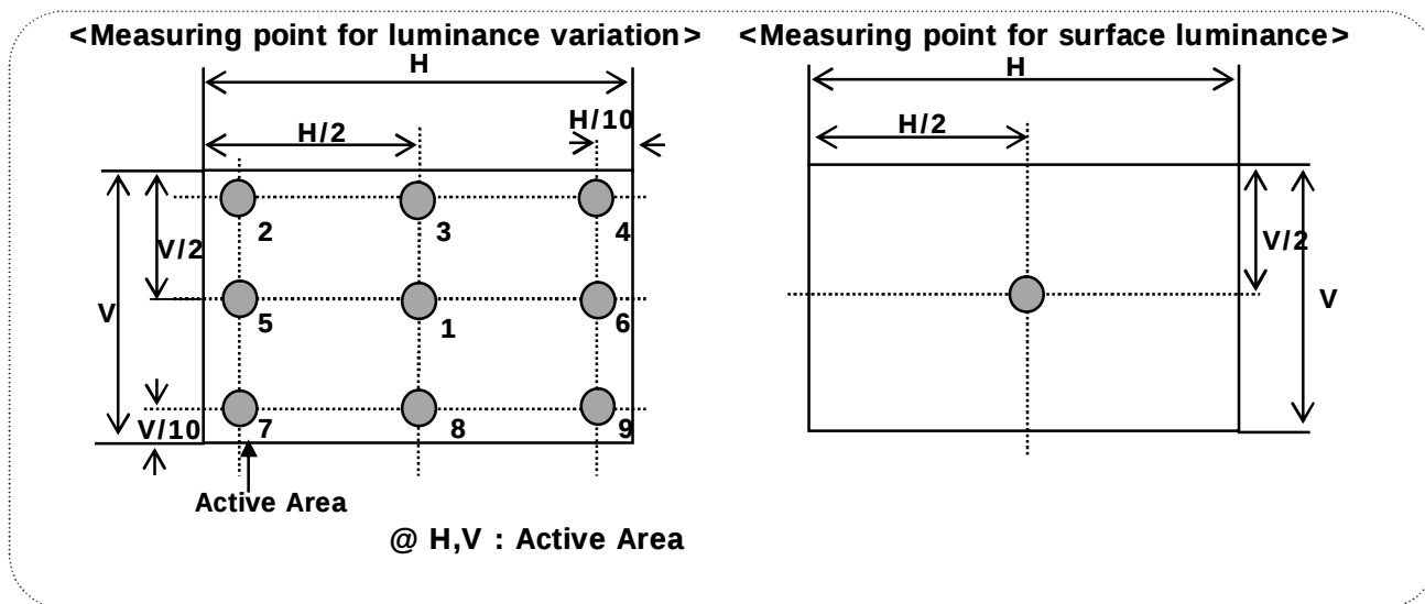
[ FIG 9 ] Measure Point for Luminance
