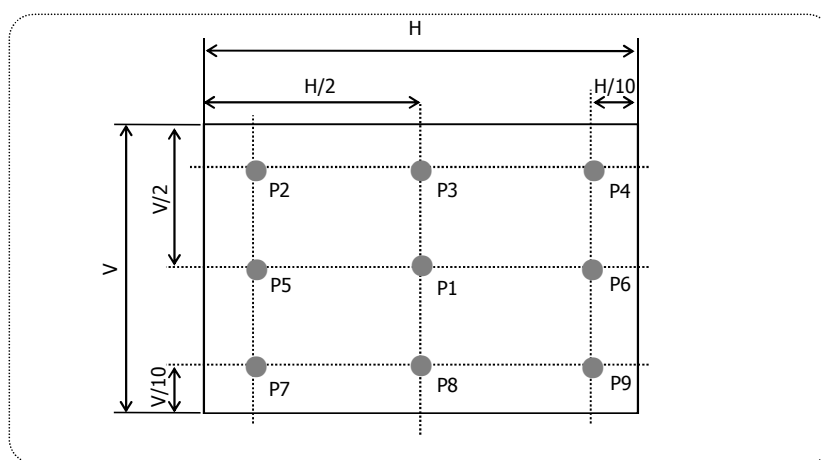
FIG.8 Measure Point for Luminance
