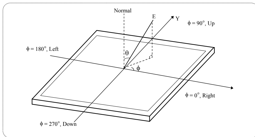
FIG.10 Viewing angle
