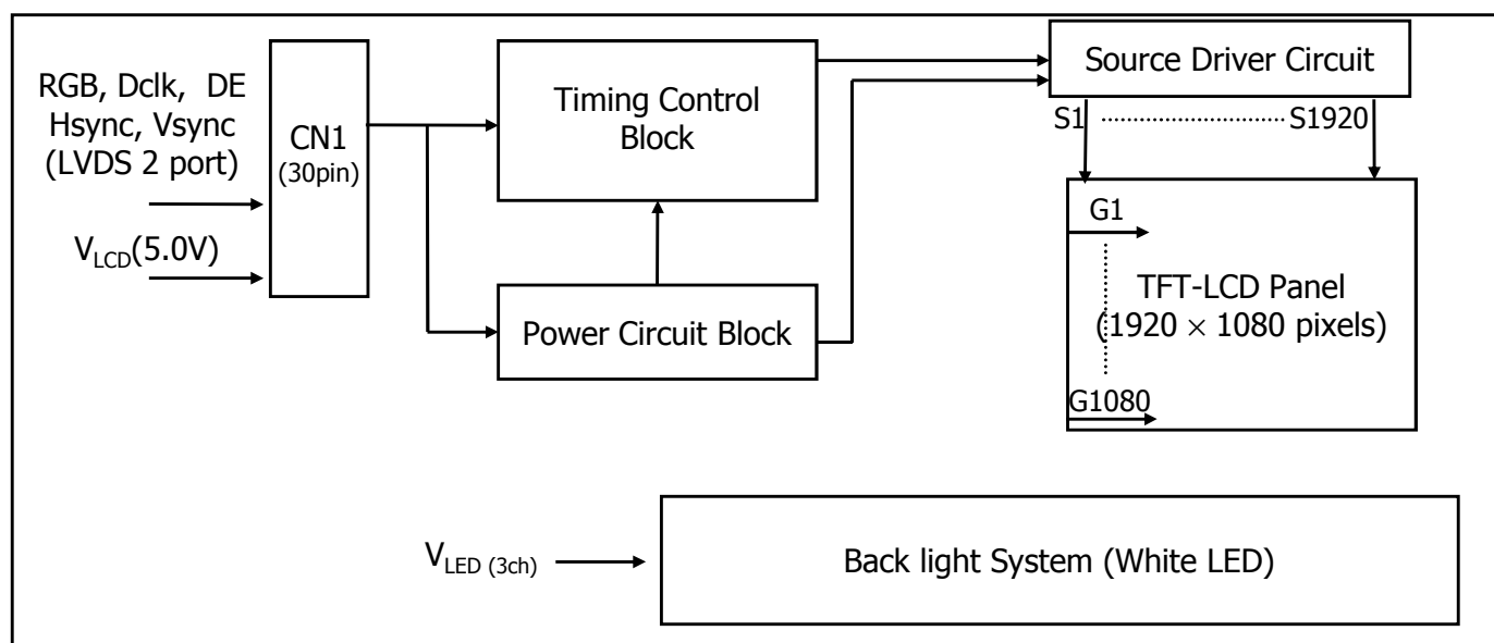
Figure 1. Block diagram
