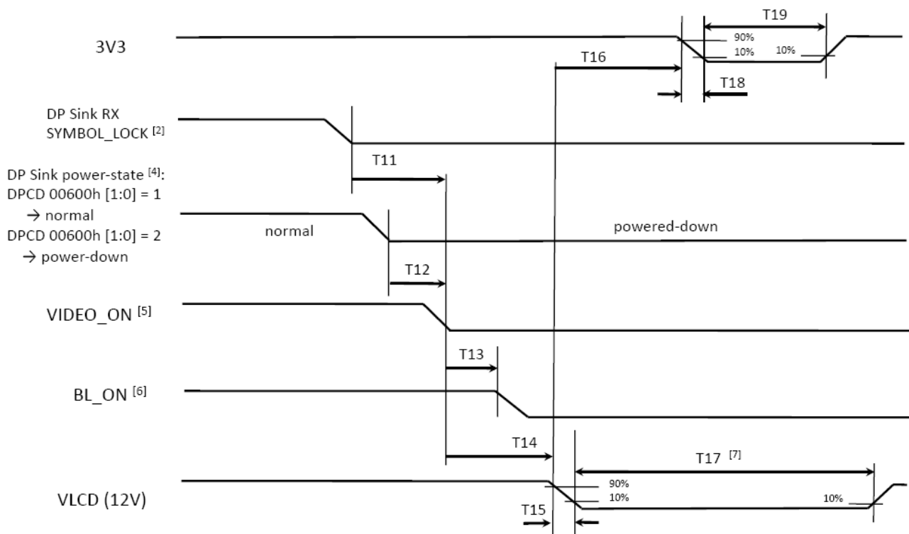
K75F Panel Power Sequence: BL_ON de-activation
