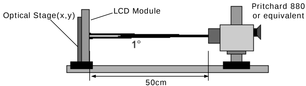
FIG. 2 Optical Characteristic Measurement Equipment and Method
