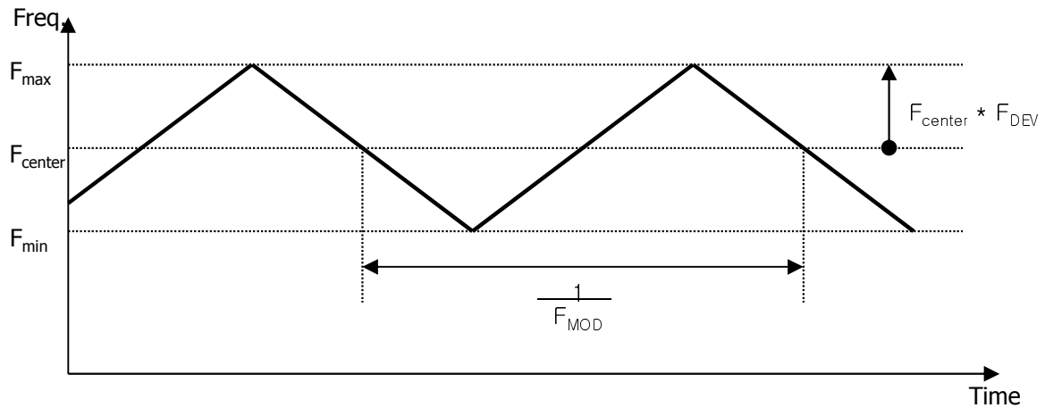
< Spread Spectrum >
