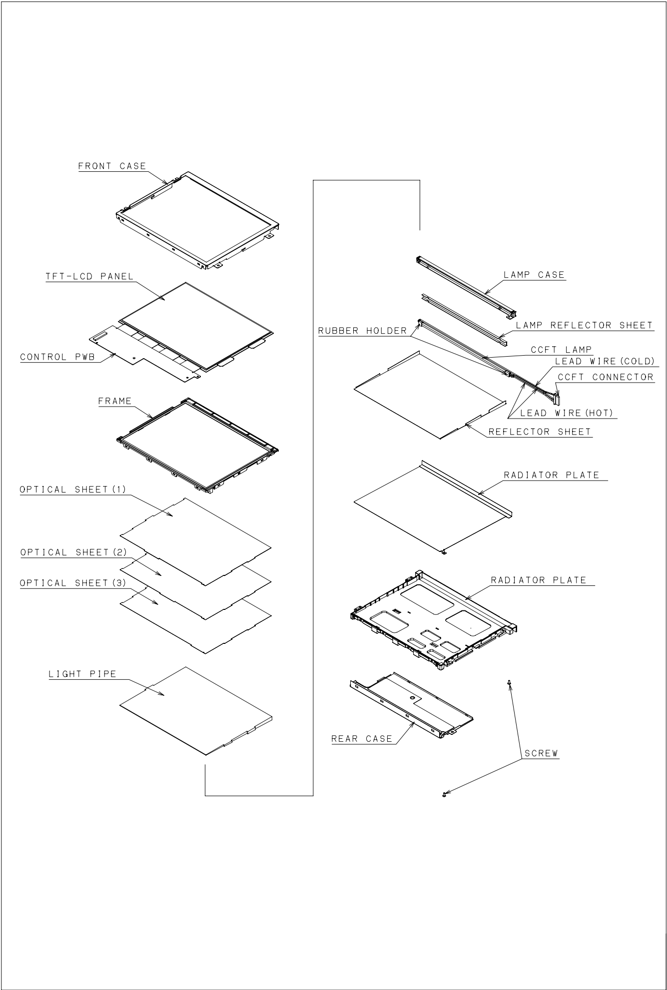
FIG.2 MODULE CONFIGUFATION
