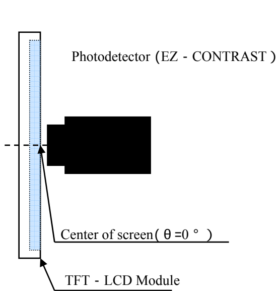
Fig3-1 Viewing angle measurement method
