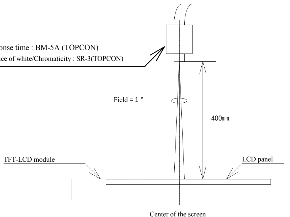
Fig.2 Optical characteristics measurement method
