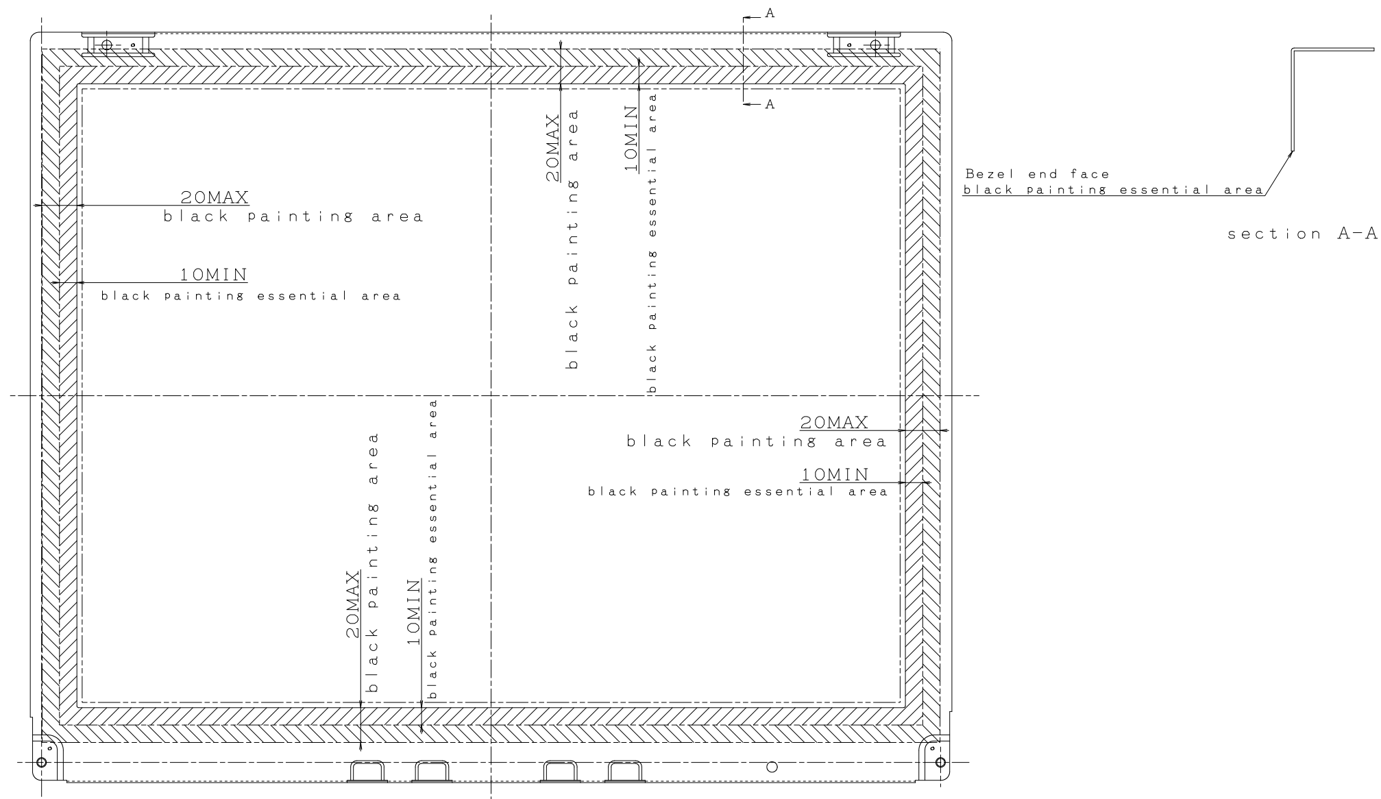
Fig2: Black painting specification
