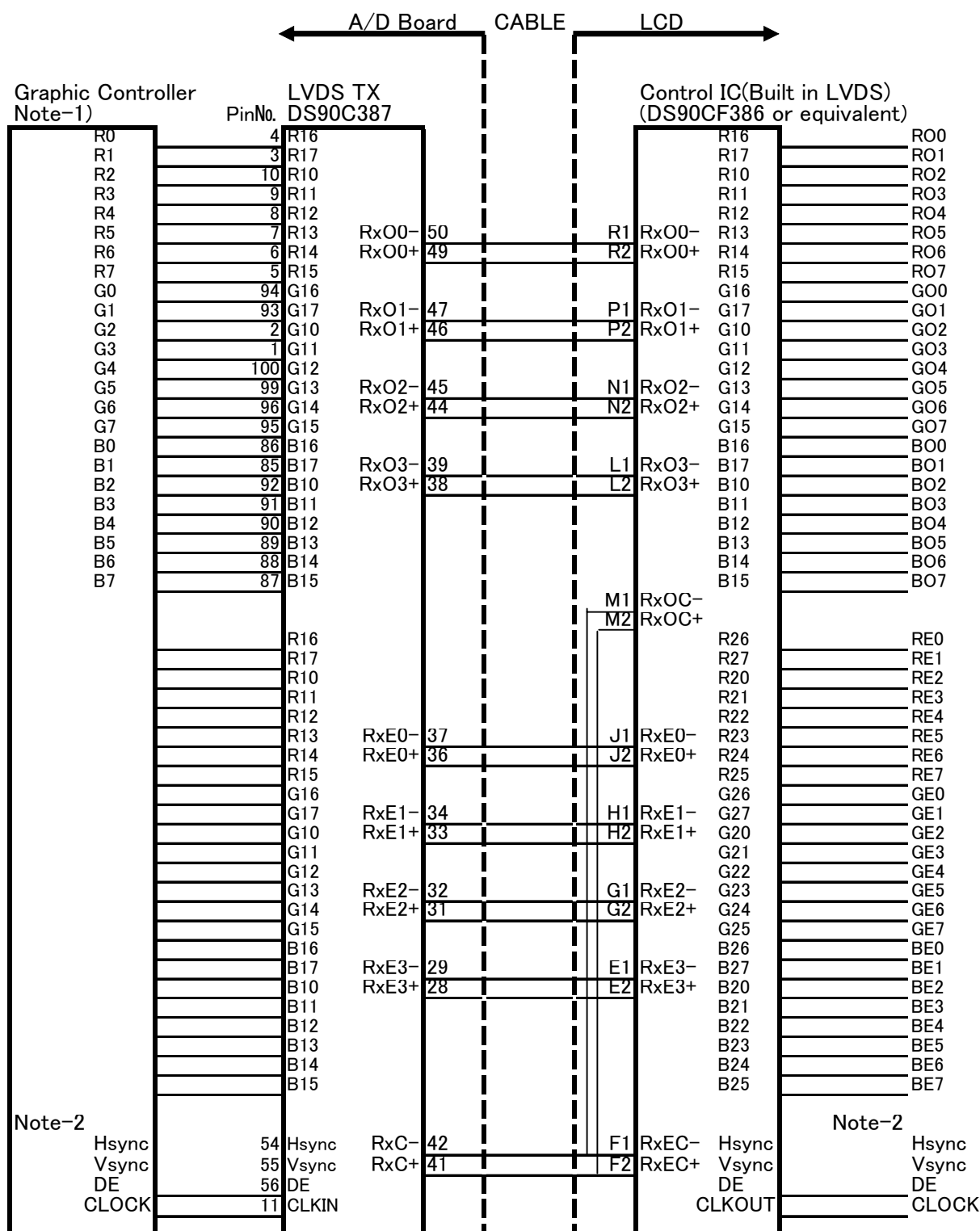
LDI Interface block diagram(Single input → Dual output)
