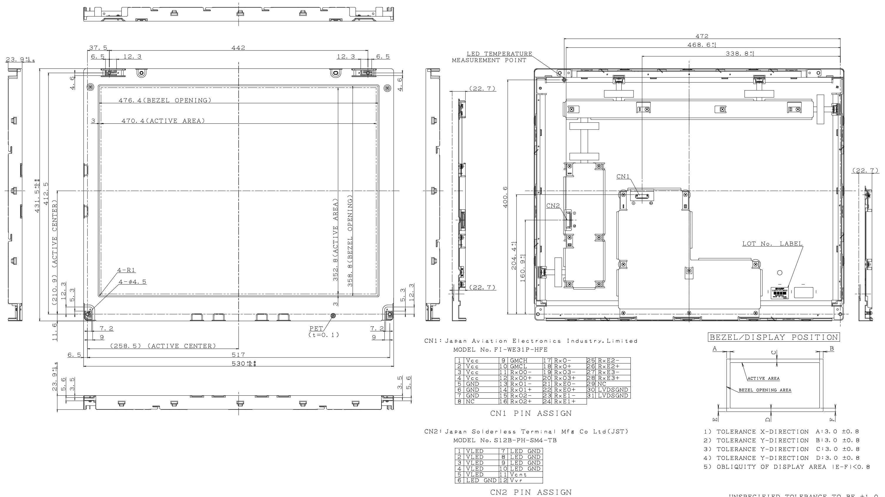
Fig 1: LQ231U1LW32 Outline dimensions
