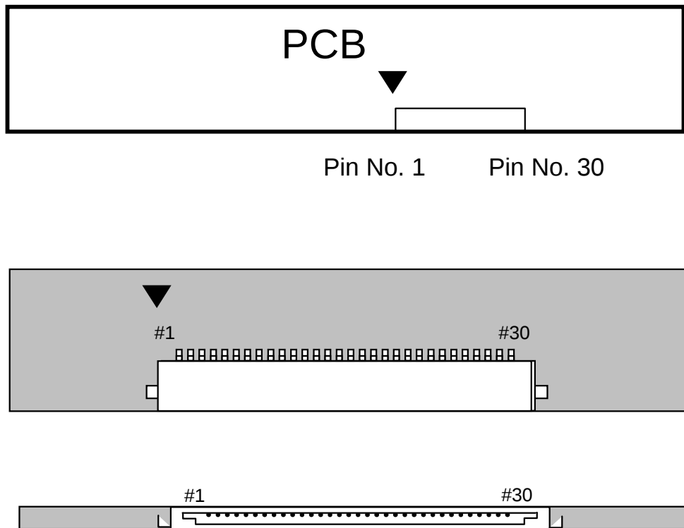
Fig. Connector diagram
