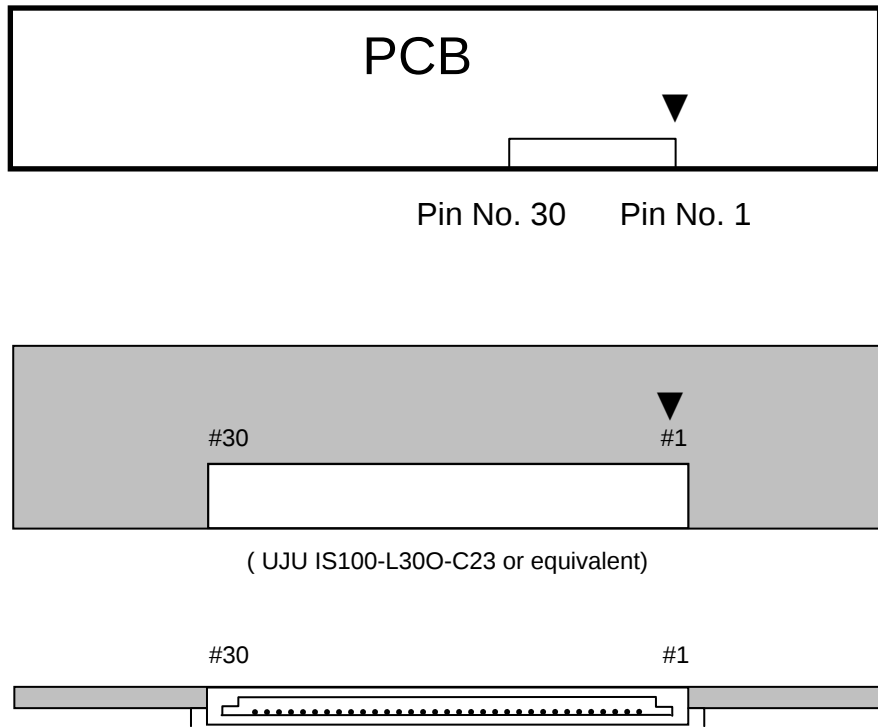
Fig. Connector diagram
