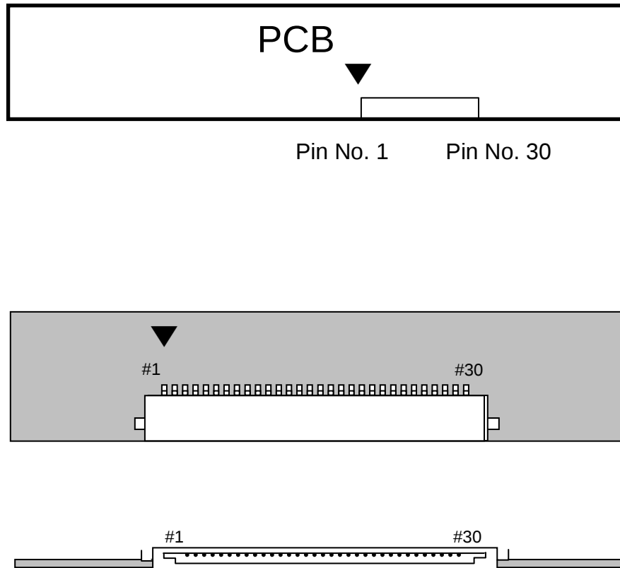
Fig. Connector diagram
