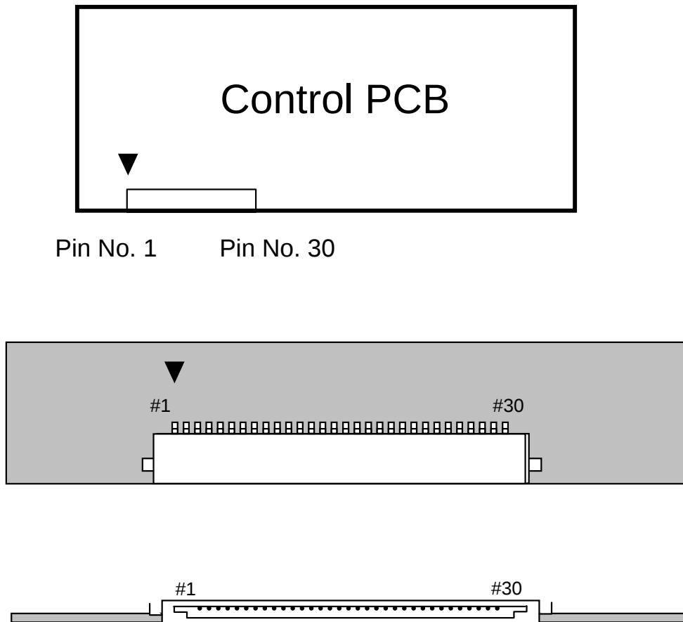
Fig. Connector diagram
