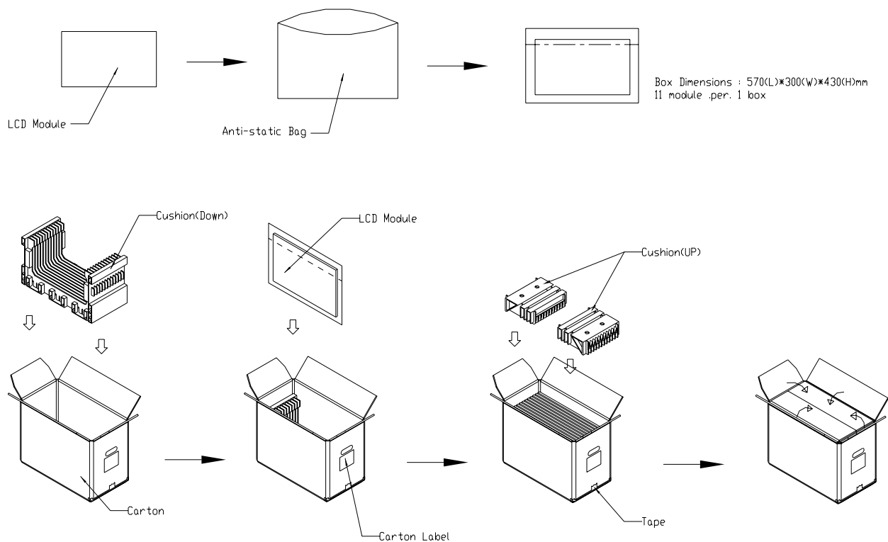
Figure. 7-1 Packing method
