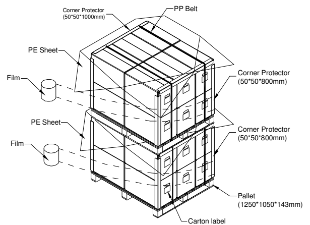
Figure. 8-2 Packing method
