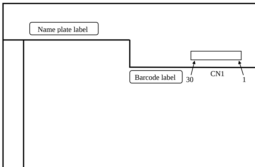
Rear view
