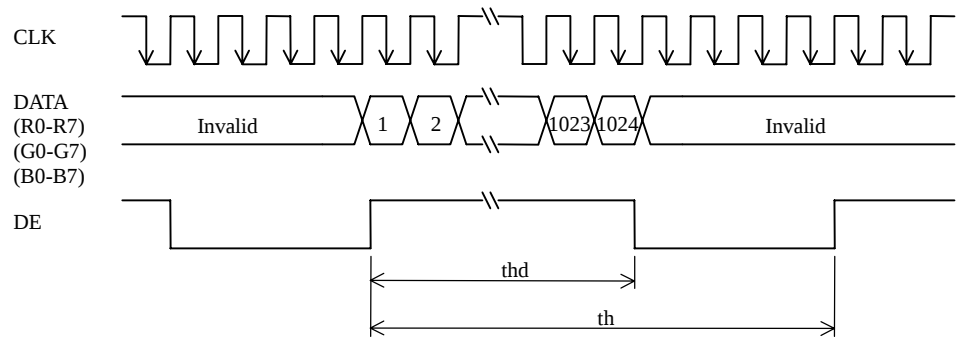
Horizontal timing
