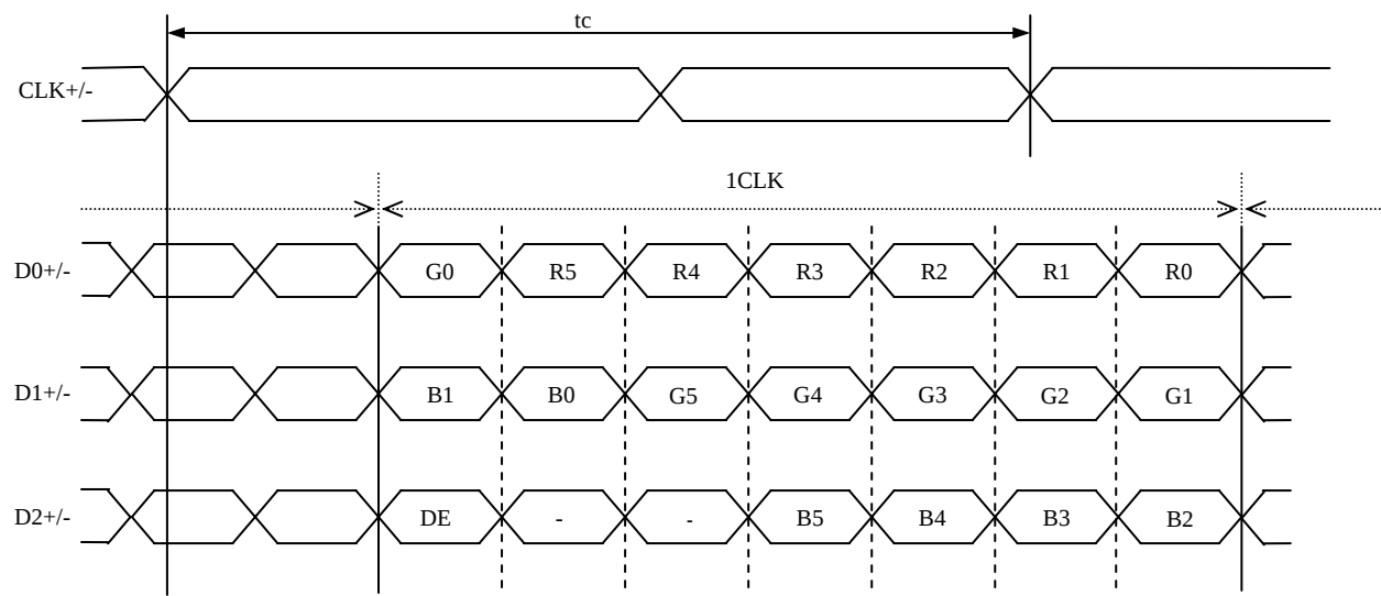
(3) Input data signal: 6bit
