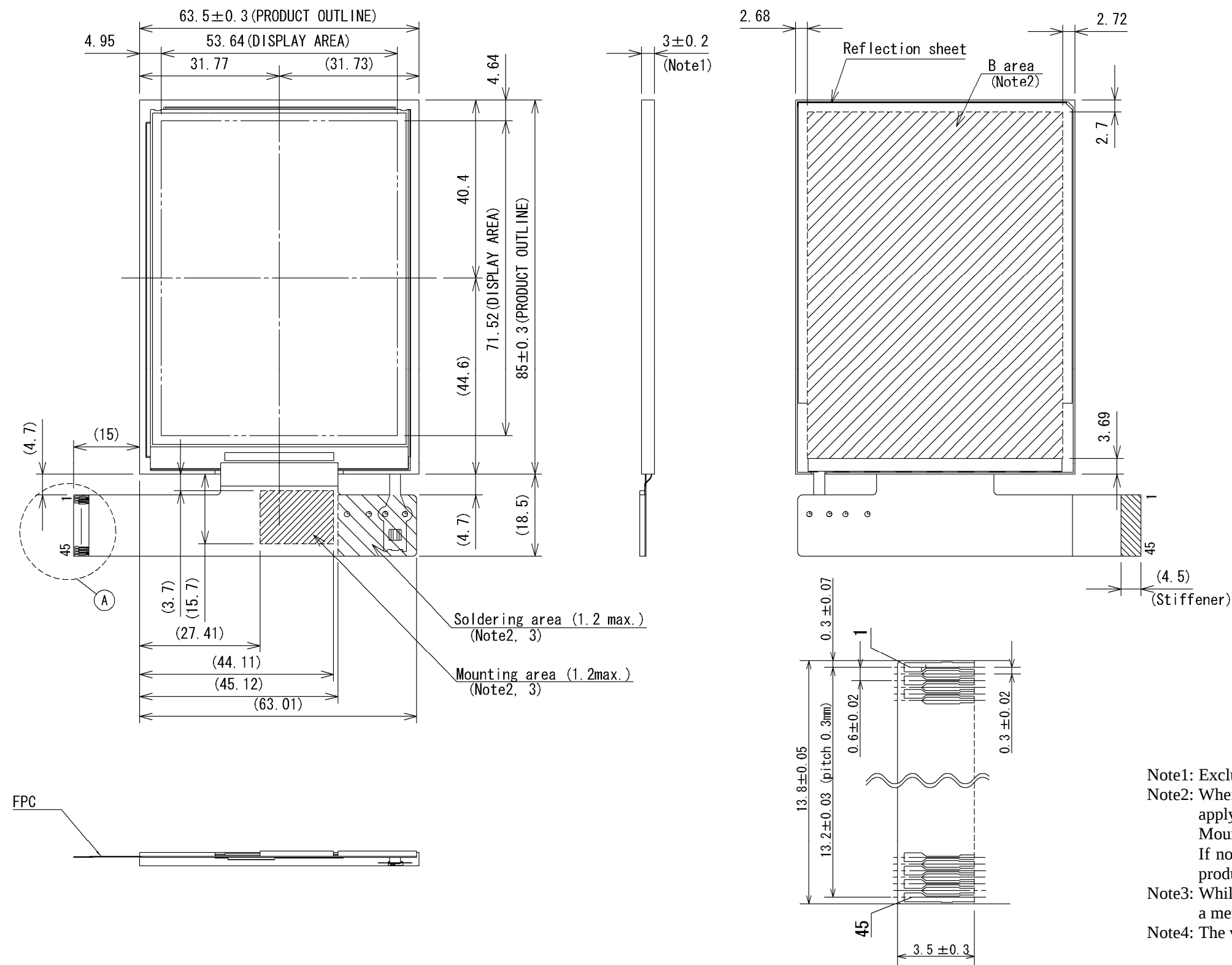
Adaptable connector:FH23-45S-0.3SHW(05) (HRS) Detail A
