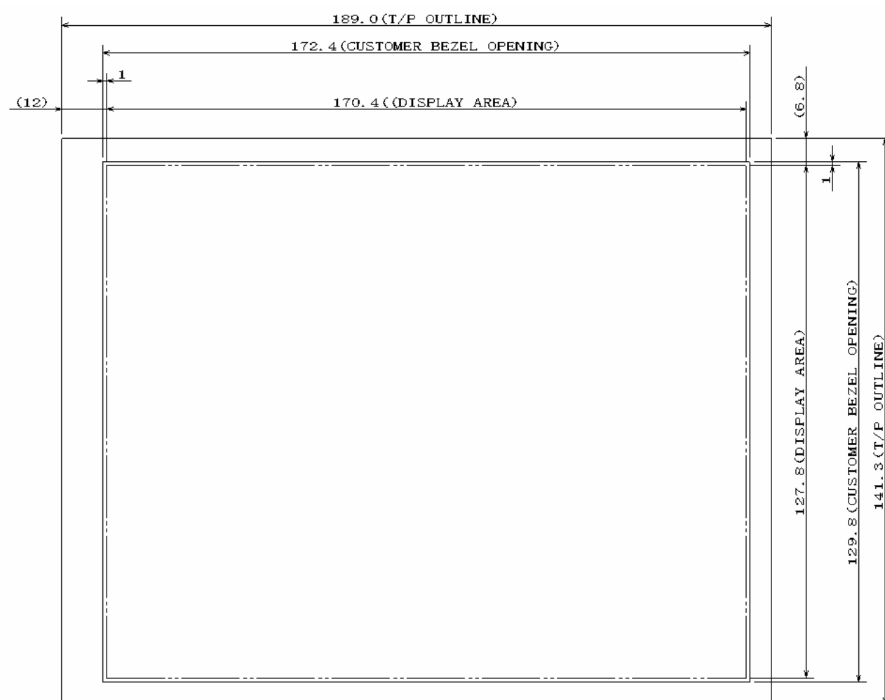
Customer Front Bezel Opening Design
