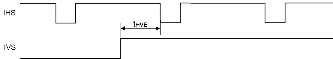
Fig. IHS and IVS waveform in even field
