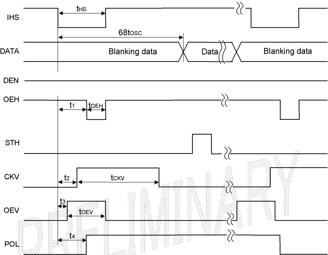
Fig.IHS and horizontal control timing waveforms in SYNC mode
