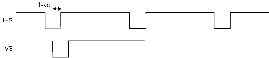
Fig. IHS and IVS waveform in odd field
