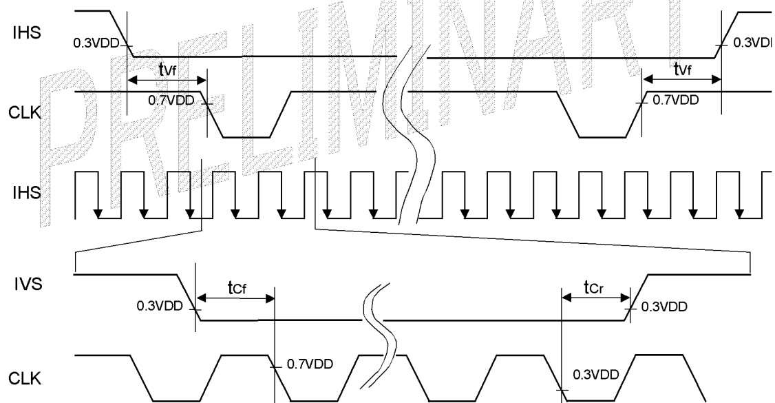
Fig. IHS and IVS timing waveform
