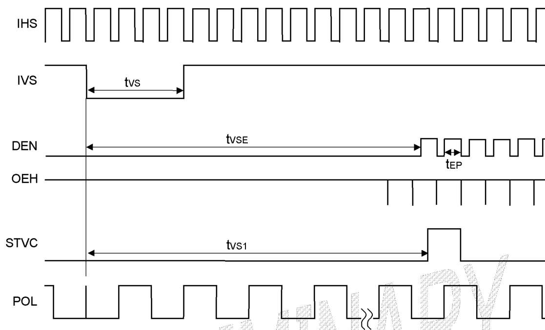
Fig. IHS and vertical control timing waveform
