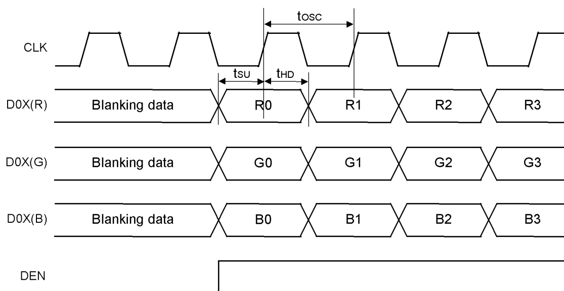
Fig. CLK,DATA and DEN waveform in Digital Parallel RGB
