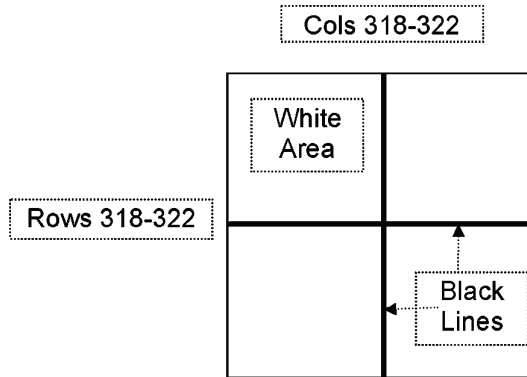
TEST PATTERN FOR IMAGE STICKING TEST
