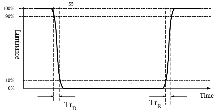
Fig.4-4 Response time
